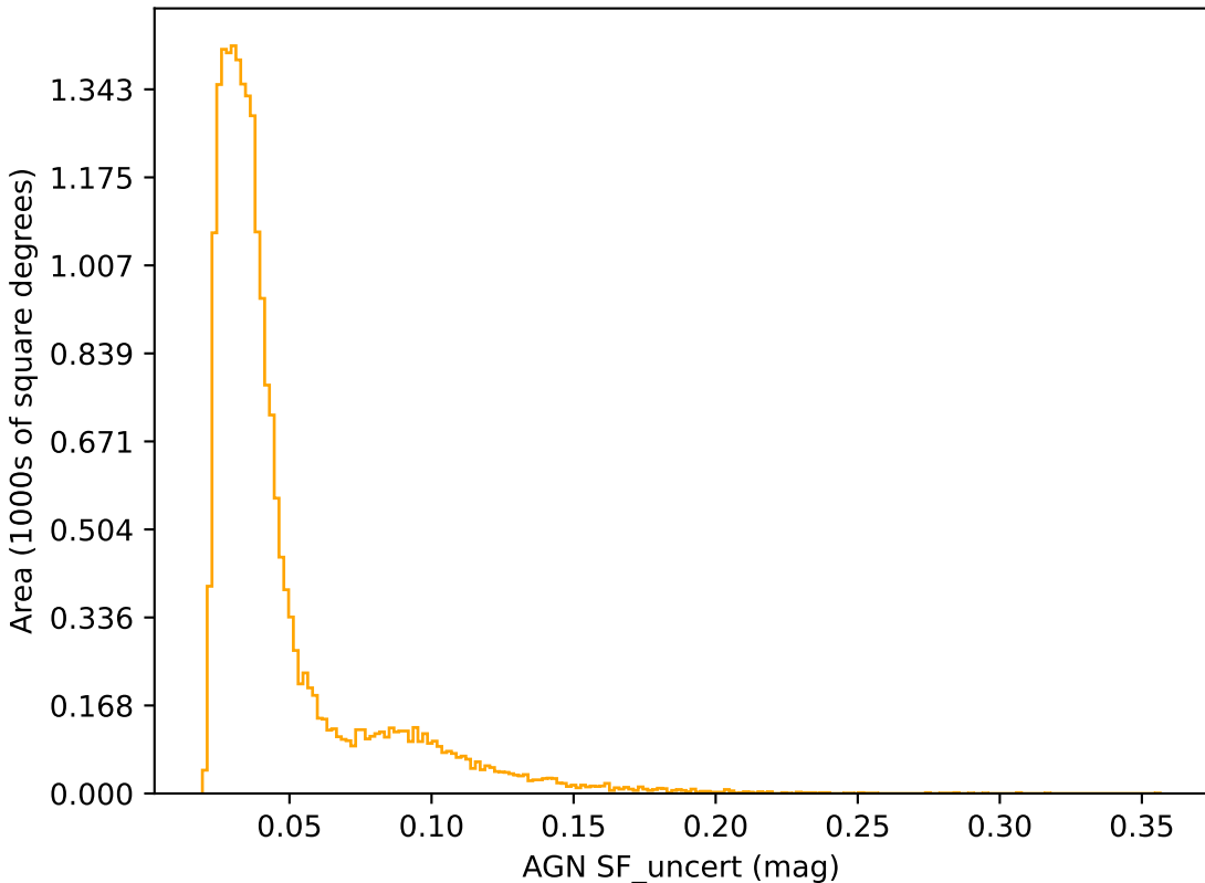
mw_roll_bulge_v3.3_10yrs r band: AGN SF_uncert
