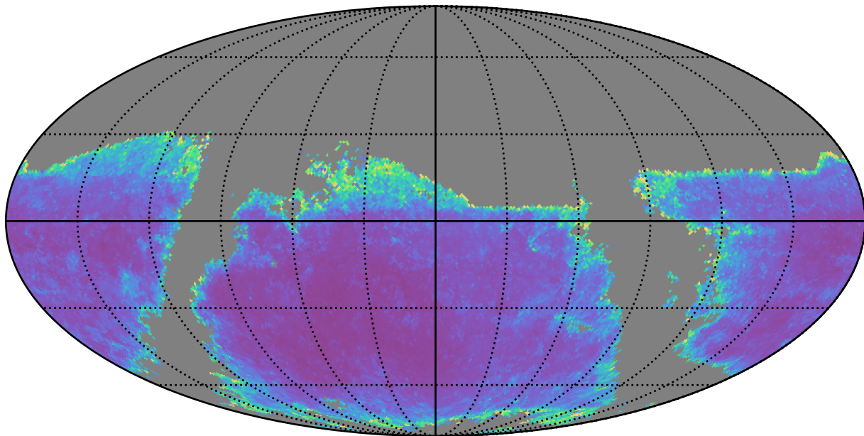
mw_roll_bulge_v3.3_10yrs g band: AGN SF_uncert
