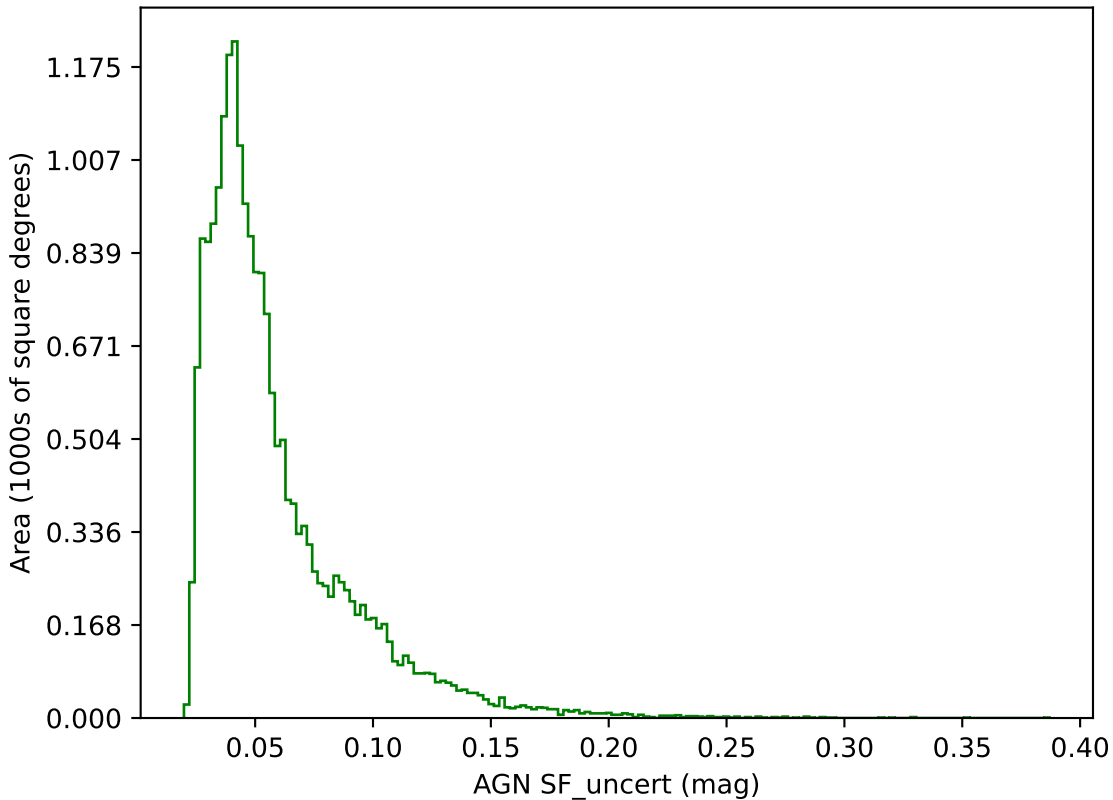
mw_roll_bulge_v3.3_10yrs g band: AGN SF_uncert
