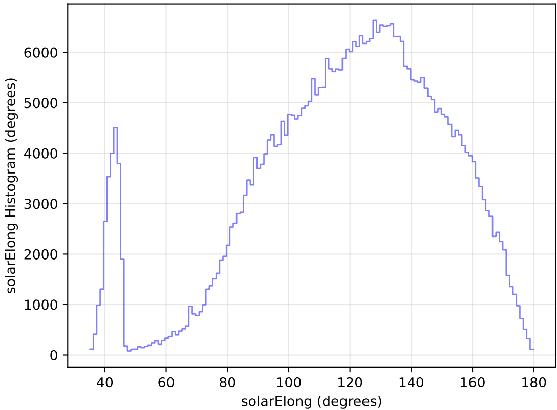
mw_roll_bulge_v3.3_10yrs WFD z band: solarElong Histogram
