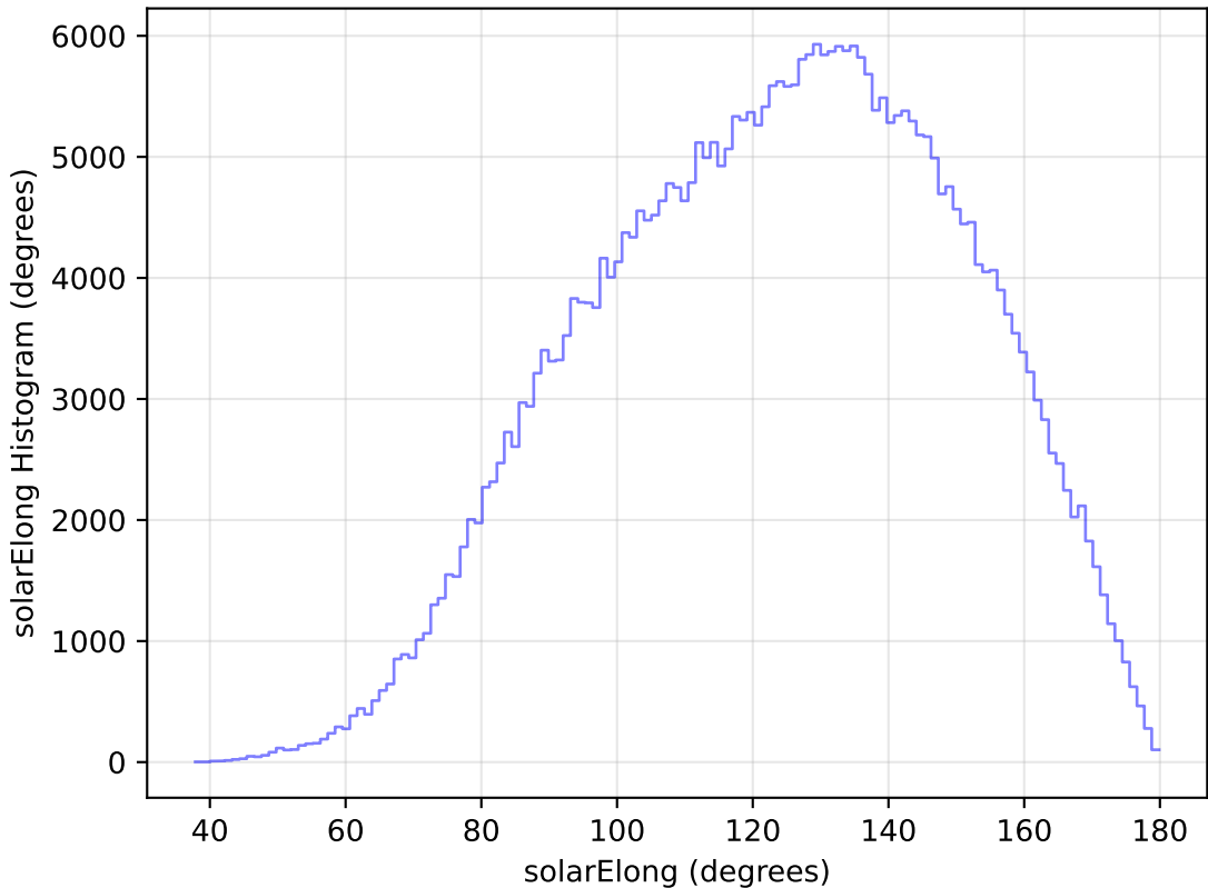
mw_roll_bulge_v3.3_10yrs WFD y band: solarElong Histogram
