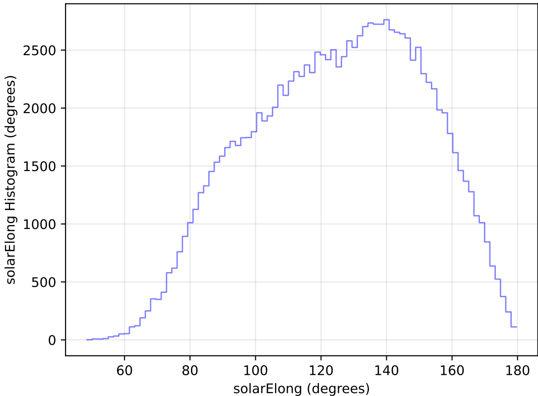
mw_roll_bulge_v3.3_10yrs WFD u band: solarElong Histogram
