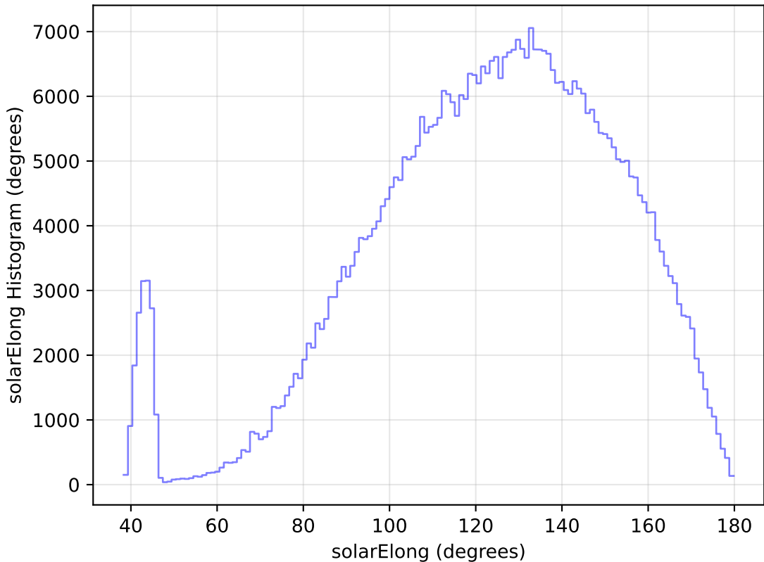
mw_roll_bulge_v3.3_10yrs WFD r band: solarElong Histogram
