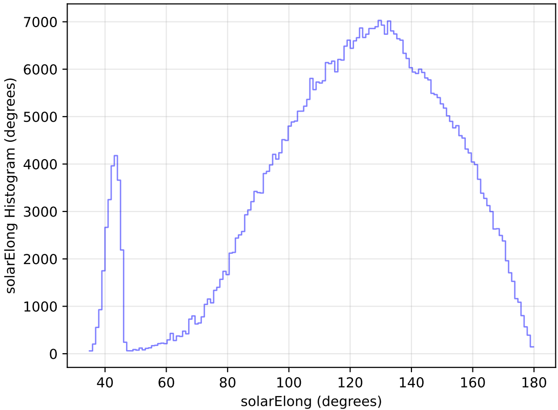
mw_roll_bulge_v3.3_10yrs WFD i band: solarElong Histogram
