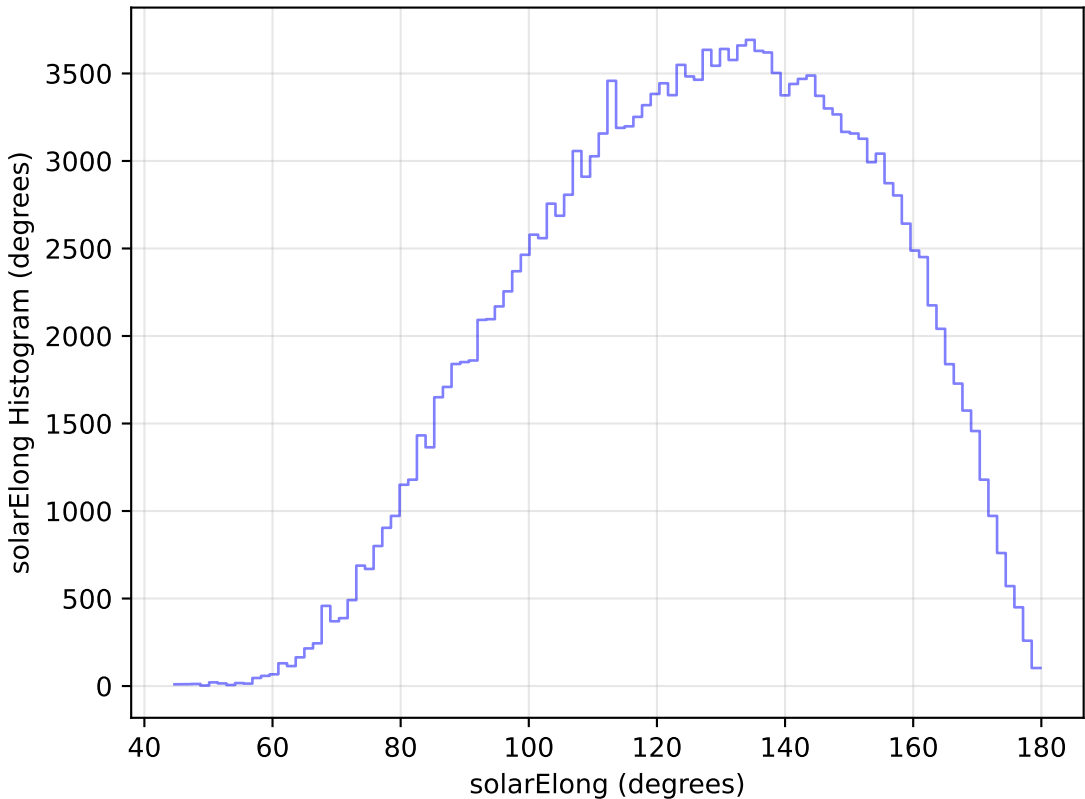
mw_roll_bulge_v3.3_10yrs WFD g band: solarElong Histogram
