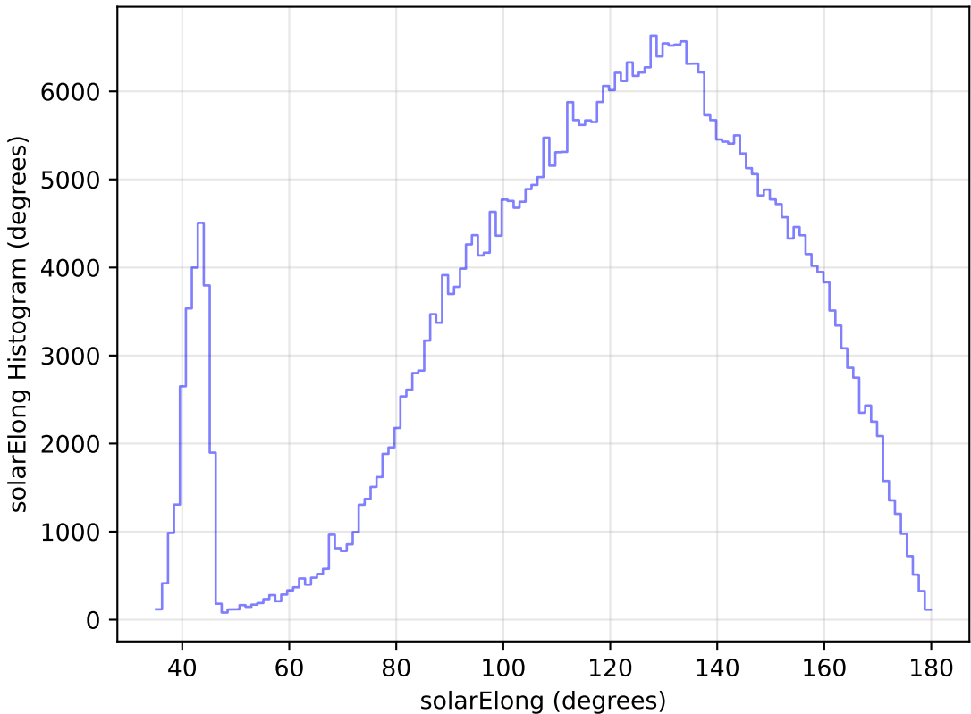
mw_roll_bulge_v3.3_10yrs All sky z band: solarElong Histogram
