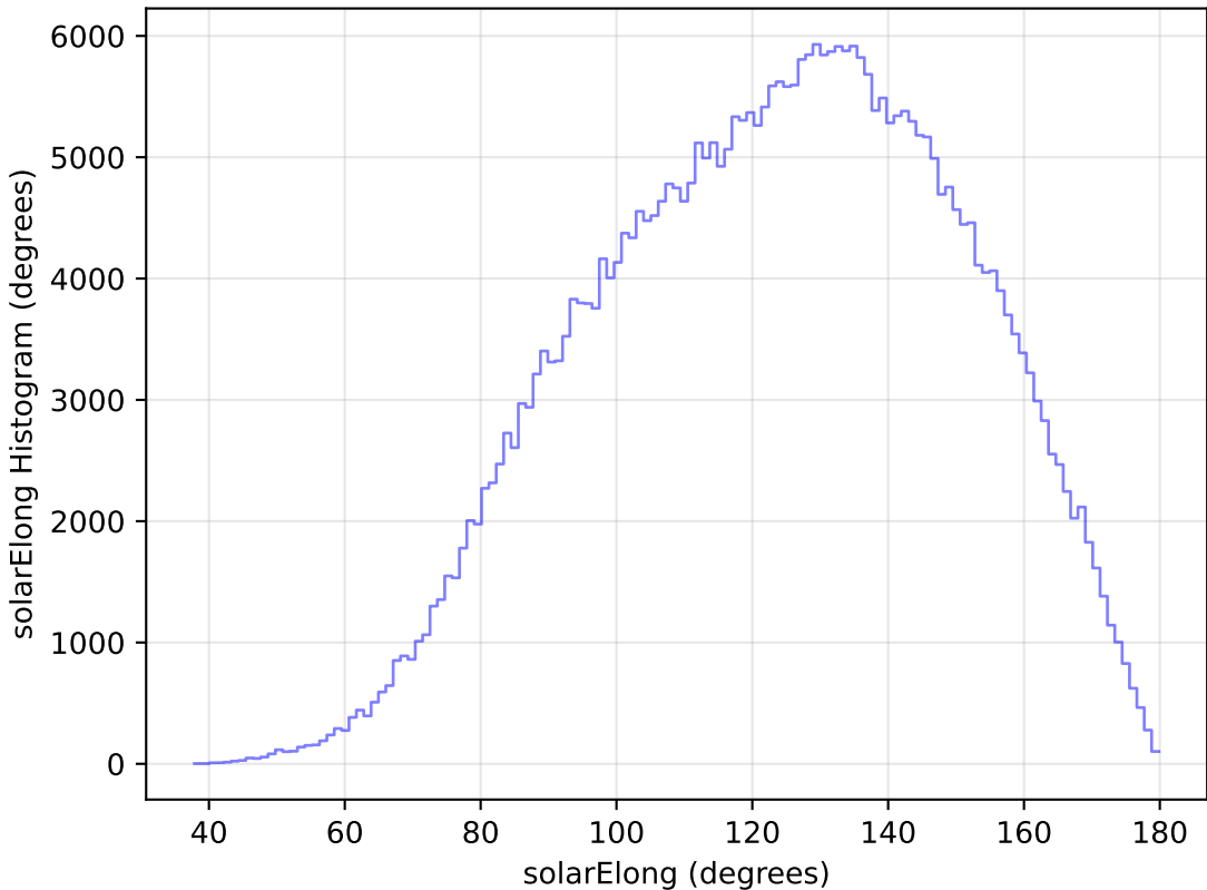
mw_roll_bulge_v3.3_10yrs All sky y band: solarElong Histogram
