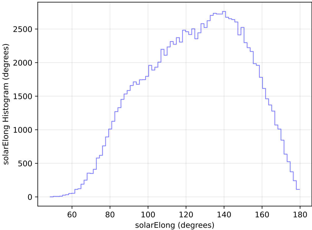
mw_roll_bulge_v3.3_10yrs All sky u band: solarElong Histogram
