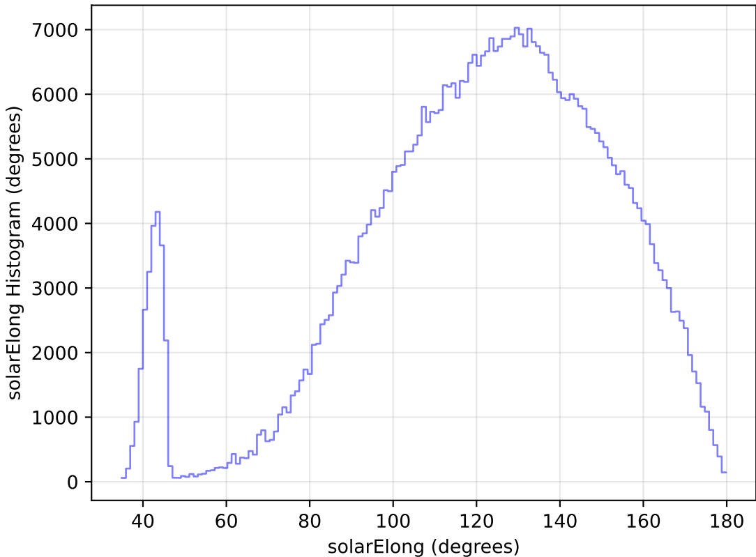
mw_roll_bulge_v3.3_10yrs All sky i band: solarElong Histogram
