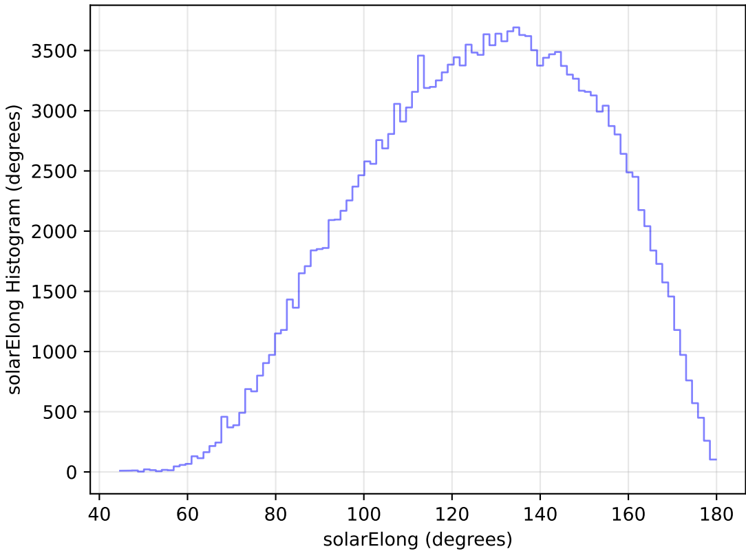
mw_roll_bulge_v3.3_10yrs All sky g band: solarElong Histogram
