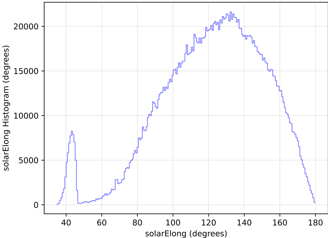
mw_roll_bulge_v3.3_10yrs All sky all bands: solarElong Histogram
