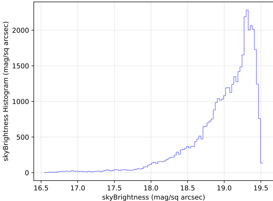
mw_roll_bulge_v3.3_10yrs Yr 1 z band: skyBrightness Histogram
