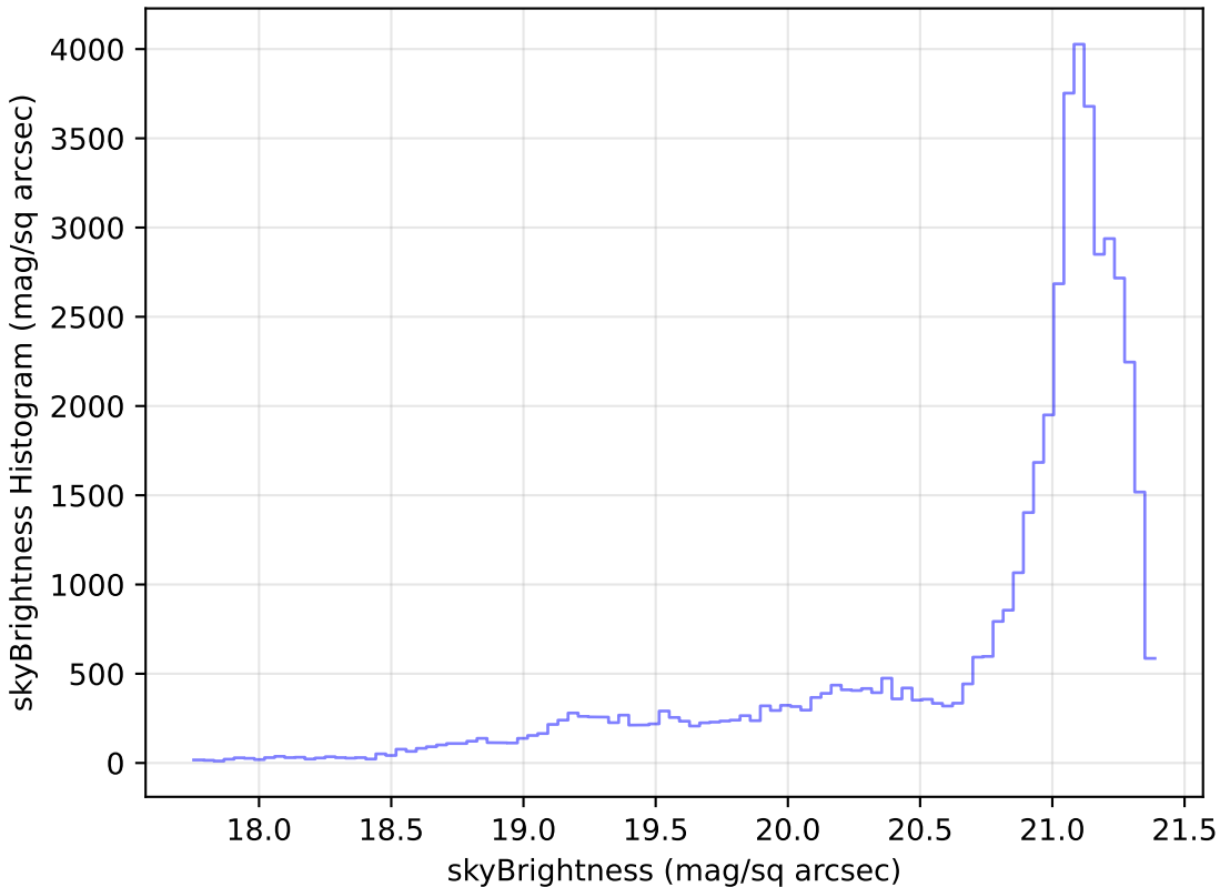
mw_roll_bulge_v3.3_10yrs Yr 1 r band: skyBrightness Histogram
