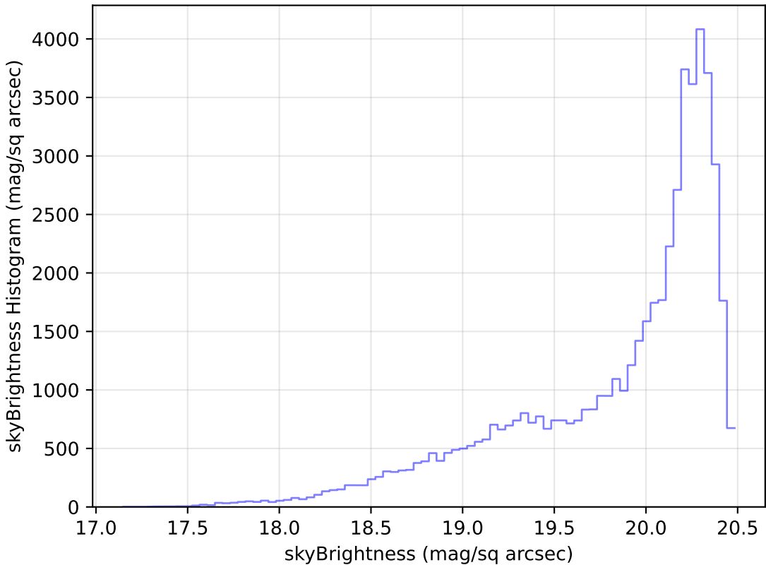
mw_roll_bulge_v3.3_10yrs Yr 1 i band: skyBrightness Histogram
