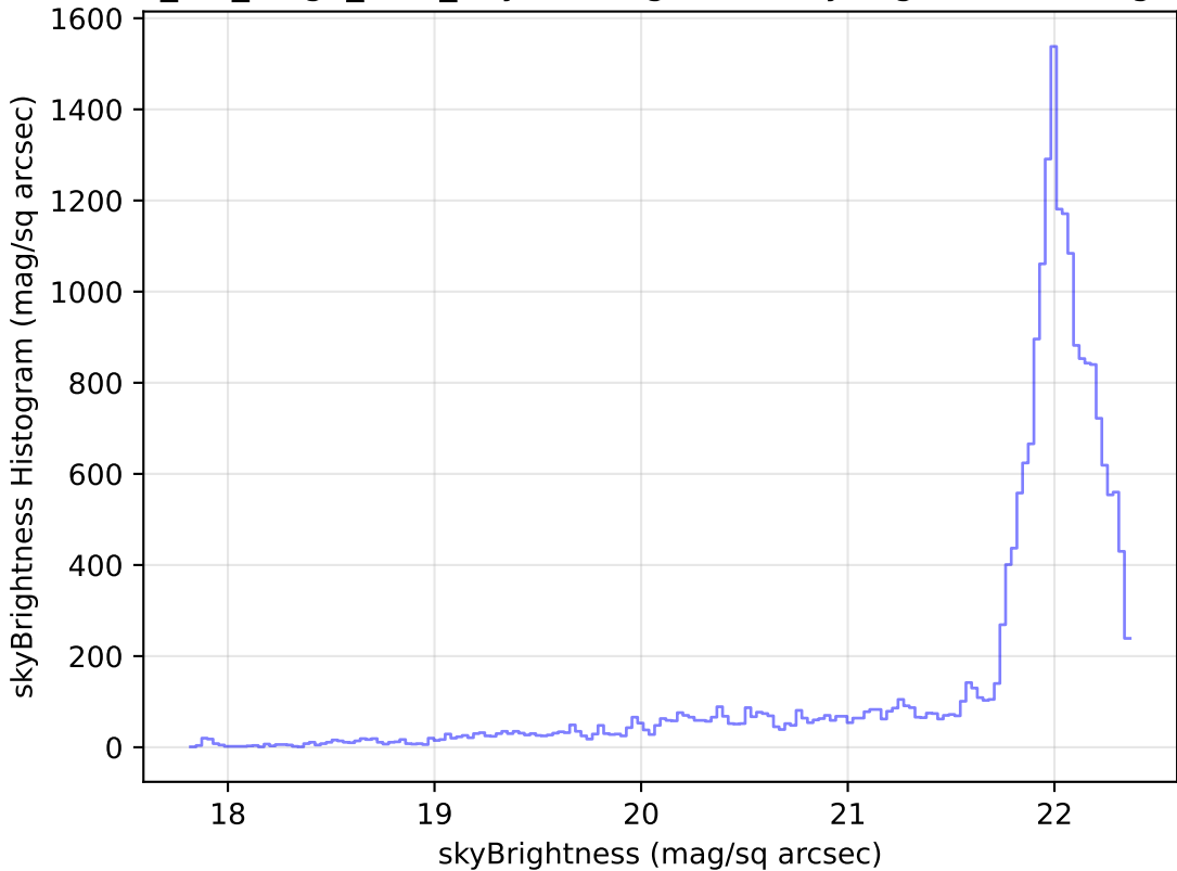
mw_roll_bulge_v3.3_10yrs Yr 1 g band: skyBrightness Histogram
