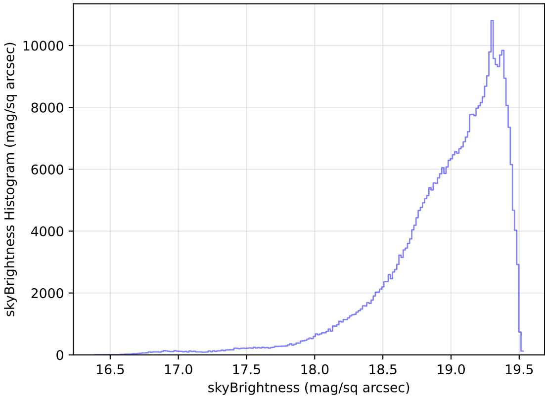
mw_roll_bulge_v3.3_10yrs WFD z band: skyBrightness Histogram
