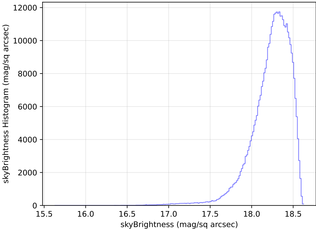
mw_roll_bulge_v3.3_10yrs WFD y band: skyBrightness Histogram
