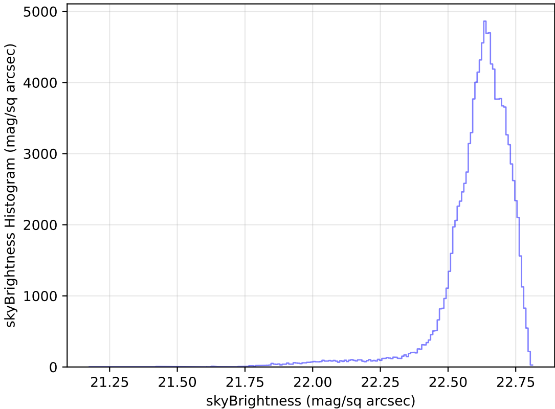
mw_roll_bulge_v3.3_10yrs WFD u band: skyBrightness Histogram
