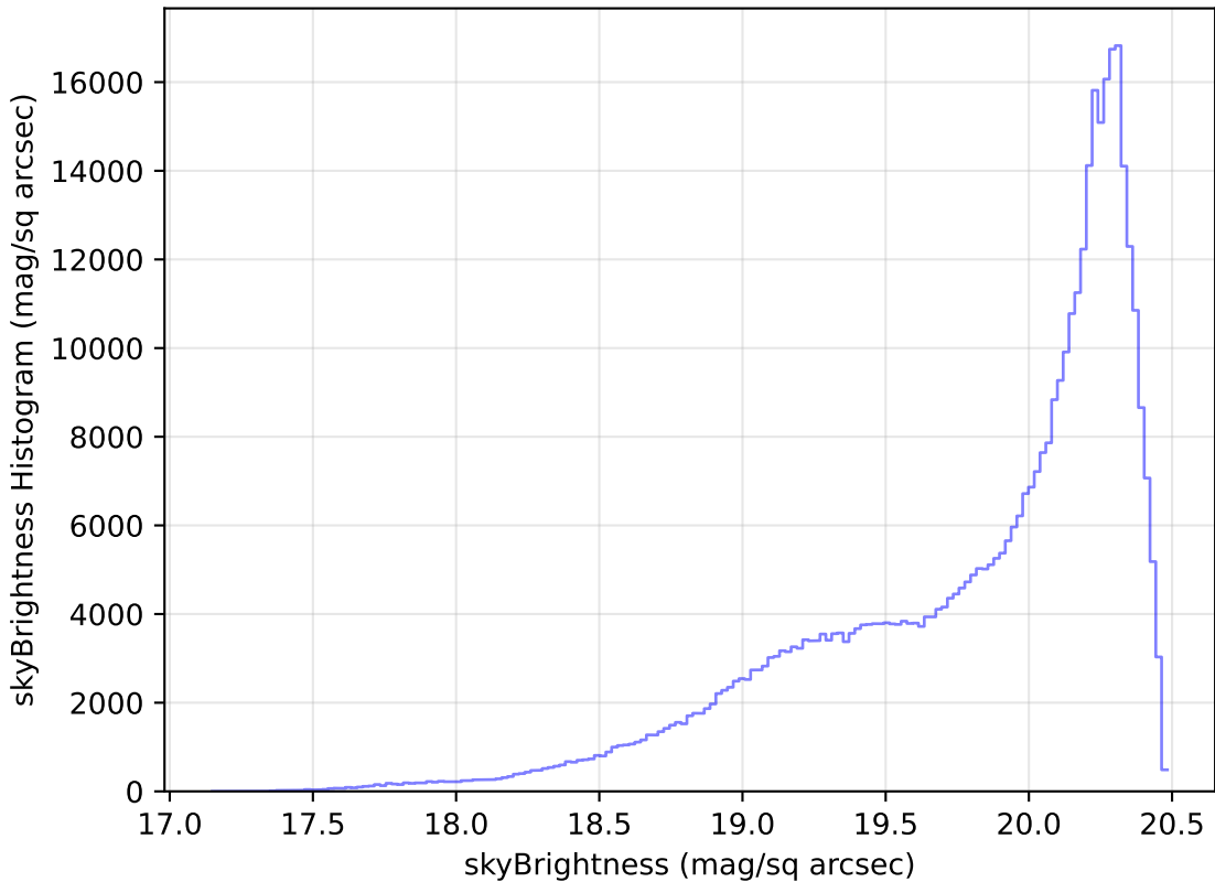
mw_roll_bulge_v3.3_10yrs WFD i band: skyBrightness Histogram
