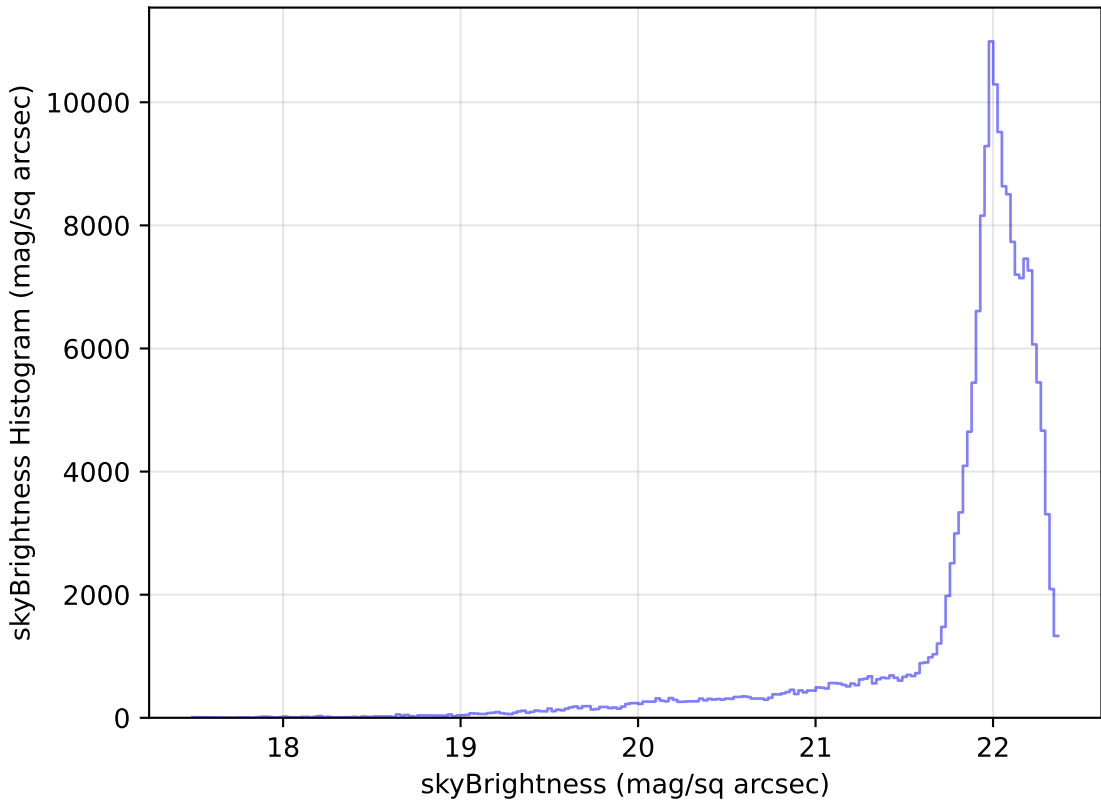
mw_roll_bulge_v3.3_10yrs WFD g band: skyBrightness Histogram
