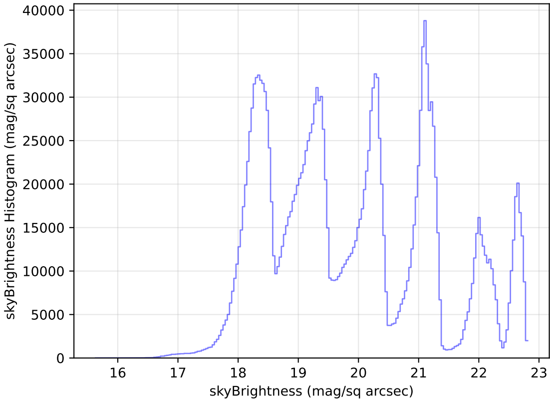
mw_roll_bulge_v3.3_10yrs WFD all bands: skyBrightness Histogram
