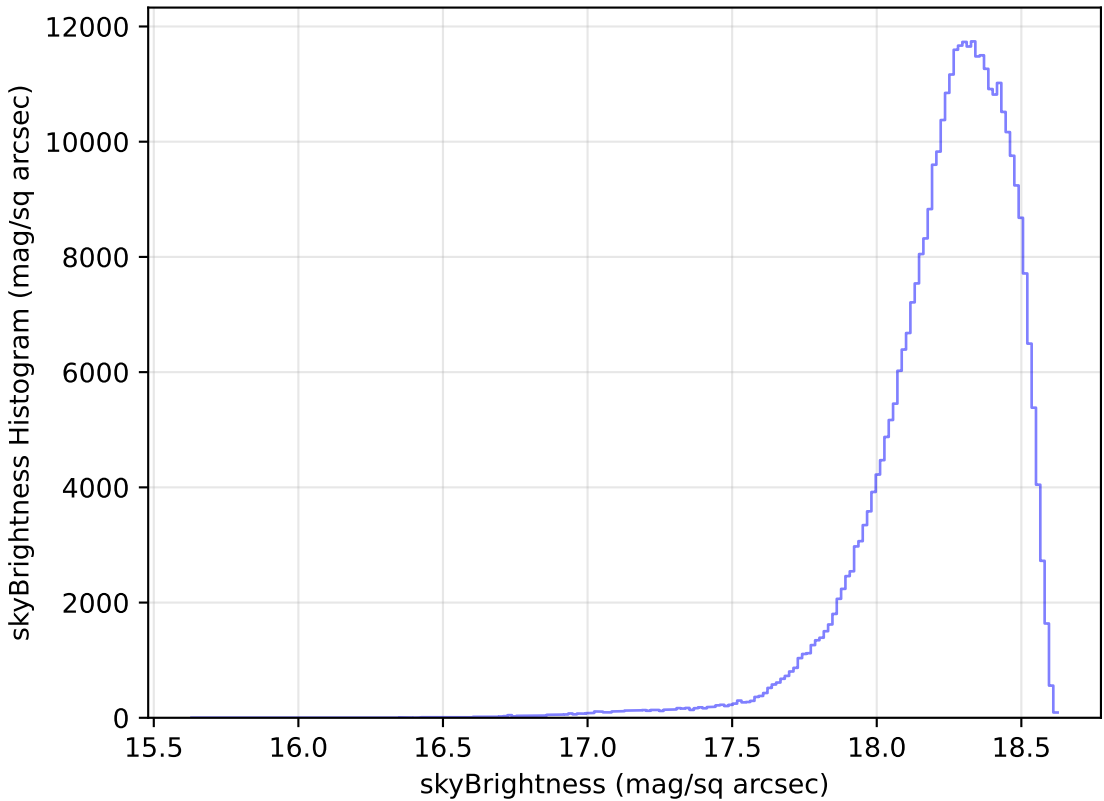
mw_roll_bulge_v3.3_10yrs All sky y band: skyBrightness Histogram
