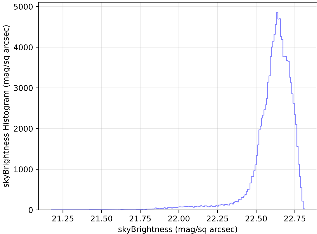
mw_roll_bulge_v3.3_10yrs All sky u band: skyBrightness Histogram
