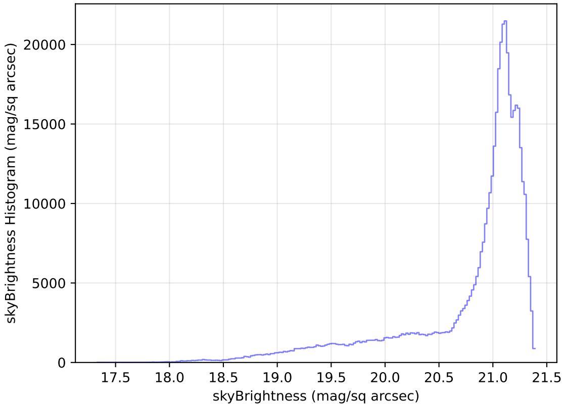
mw_roll_bulge_v3.3_10yrs All sky r band: skyBrightness Histogram
