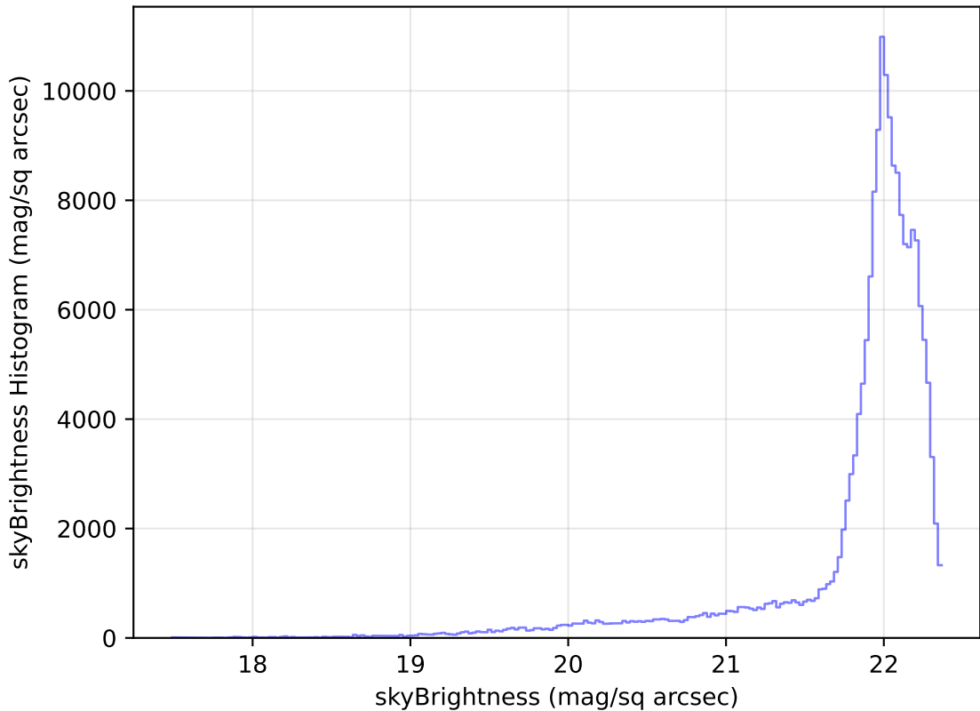
mw_roll_bulge_v3.3_10yrs All sky g band: skyBrightness Histogram
