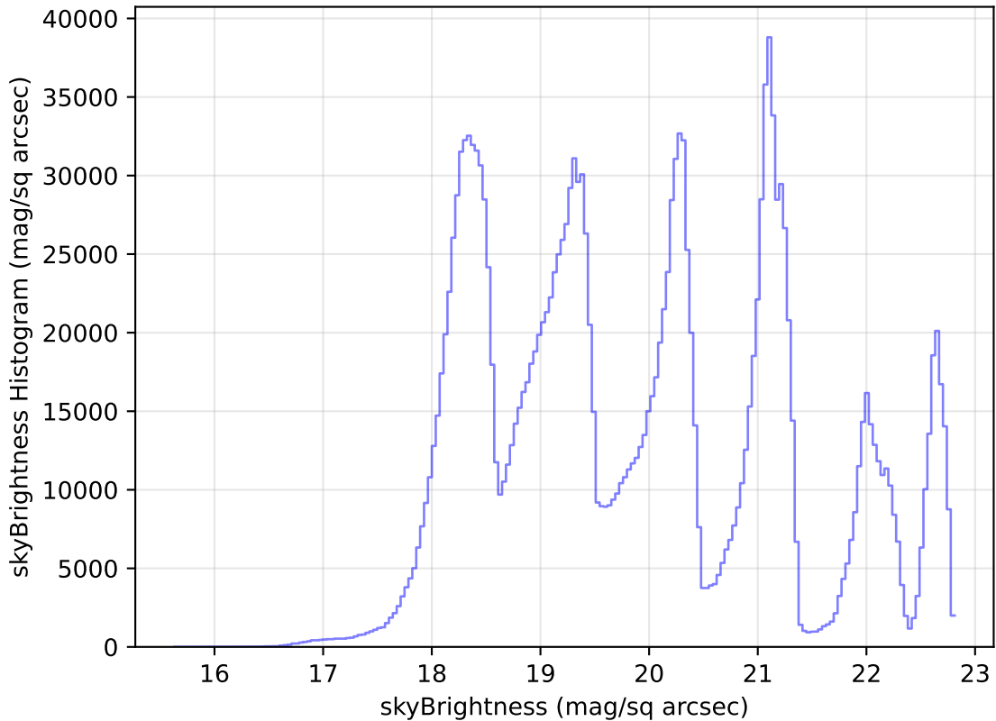
mw_roll_bulge_v3.3_10yrs All sky all bands: skyBrightness Histogram
