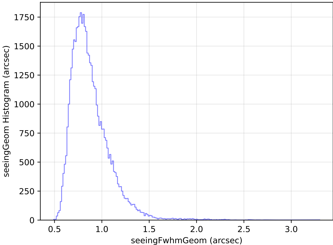
mw_roll_bulge_v3.3_10yrs Yr 1 y band: seeingGeom Histogram
