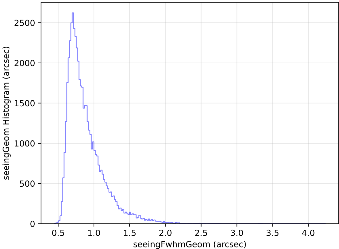
mw_roll_bulge_v3.3_10yrs Yr 1 r band: seeingGeom Histogram
