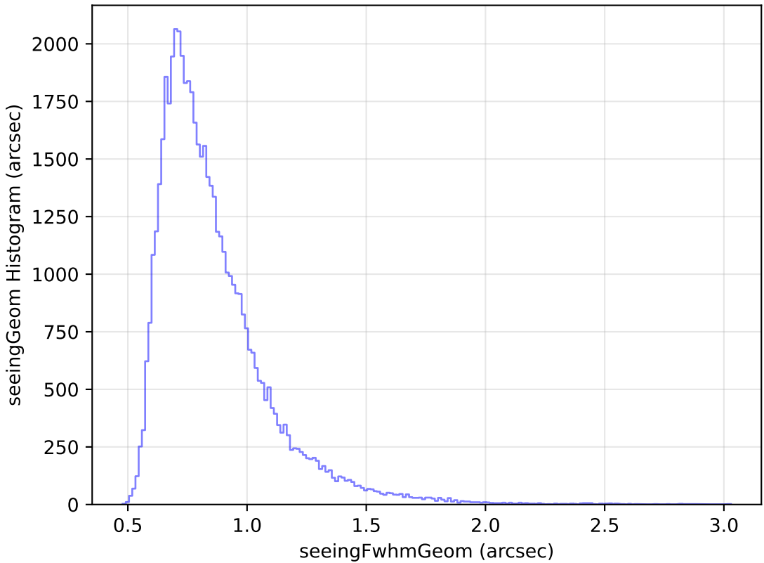
mw_roll_bulge_v3.3_10yrs Yr 1 i band: seeingGeom Histogram
