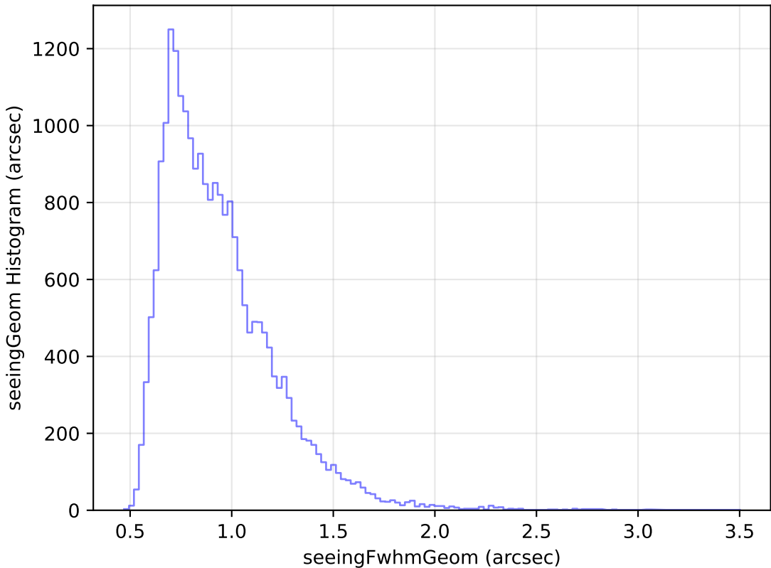
mw_roll_bulge_v3.3_10yrs Yr 1 g band: seeingGeom Histogram
