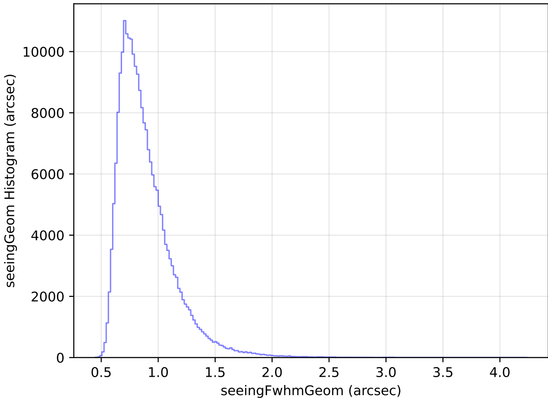
mw_roll_bulge_v3.3_10yrs Yr 1 all bands: seeingGeom Histogram
