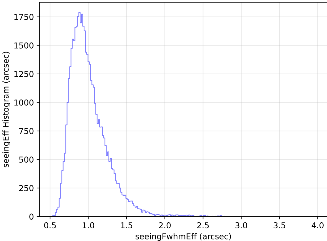
mw_roll_bulge_v3.3_10yrs Yr 1 y band: seeingEff Histogram
