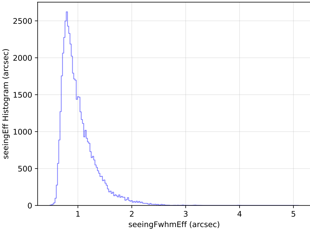
mw_roll_bulge_v3.3_10yrs Yr 1 r band: seeingEff Histogram
