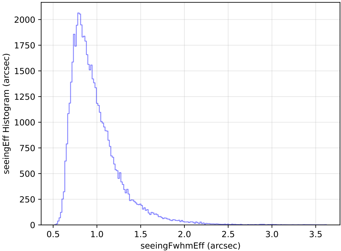
mw_roll_bulge_v3.3_10yrs Yr 1 i band: seeingEff Histogram
