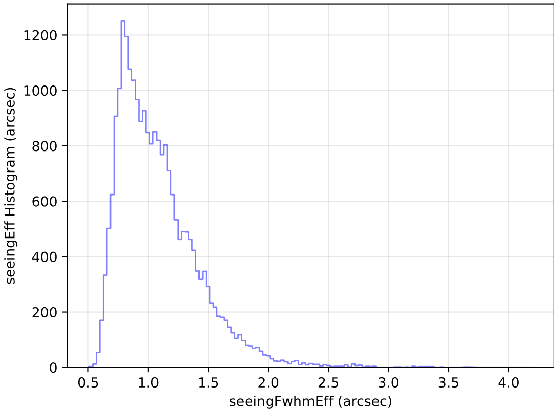
mw_roll_bulge_v3.3_10yrs Yr 1 g band: seeingEff Histogram
