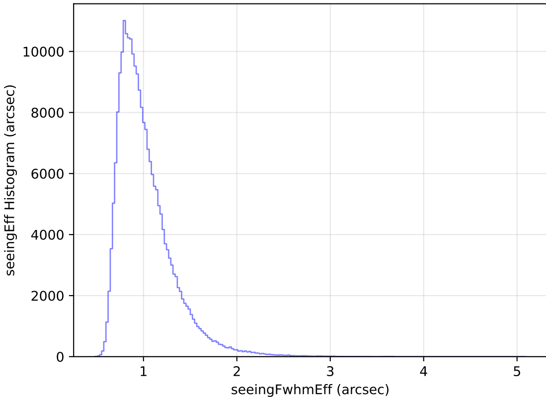
mw_roll_bulge_v3.3_10yrs Yr 1 all bands: seeingEff Histogram
