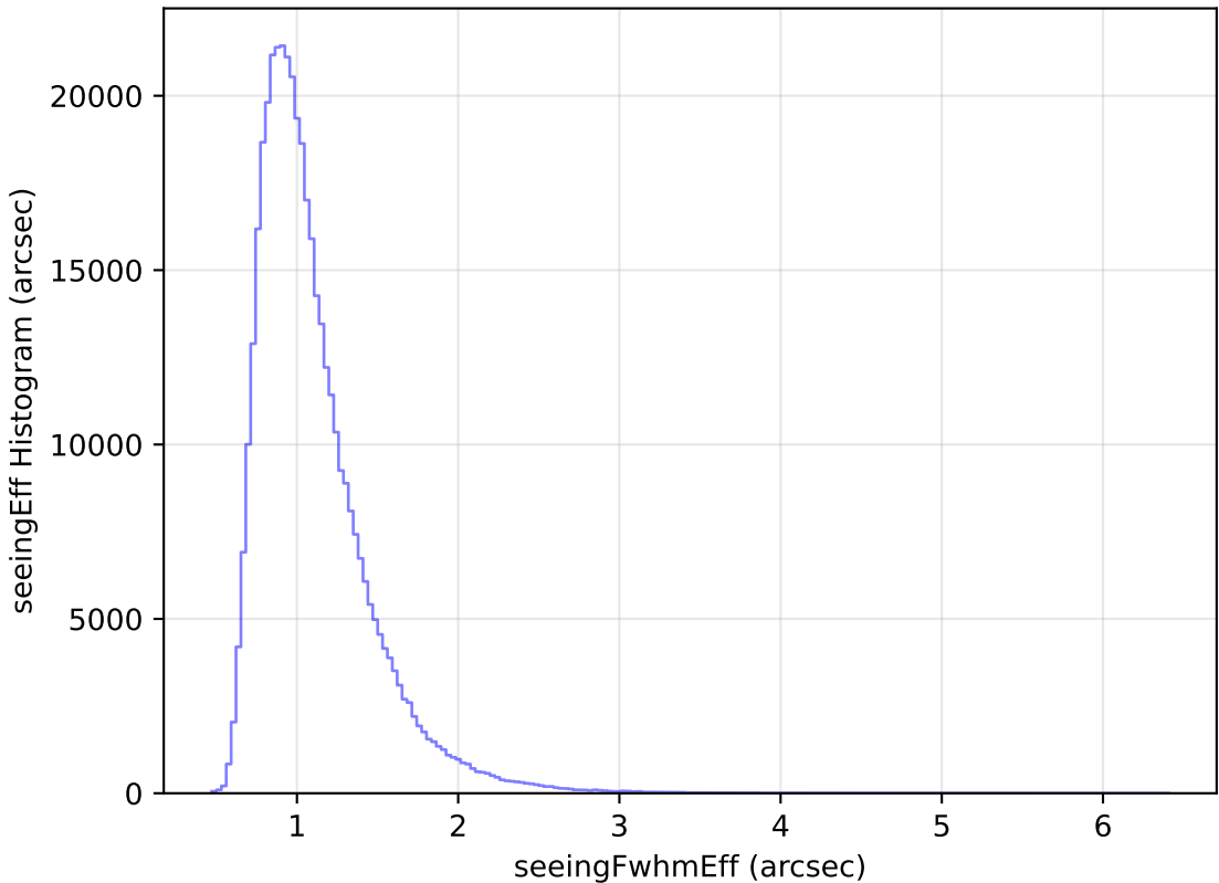
mw_roll_bulge_v3.3_10yrs WFD z band: seeingEff Histogram
