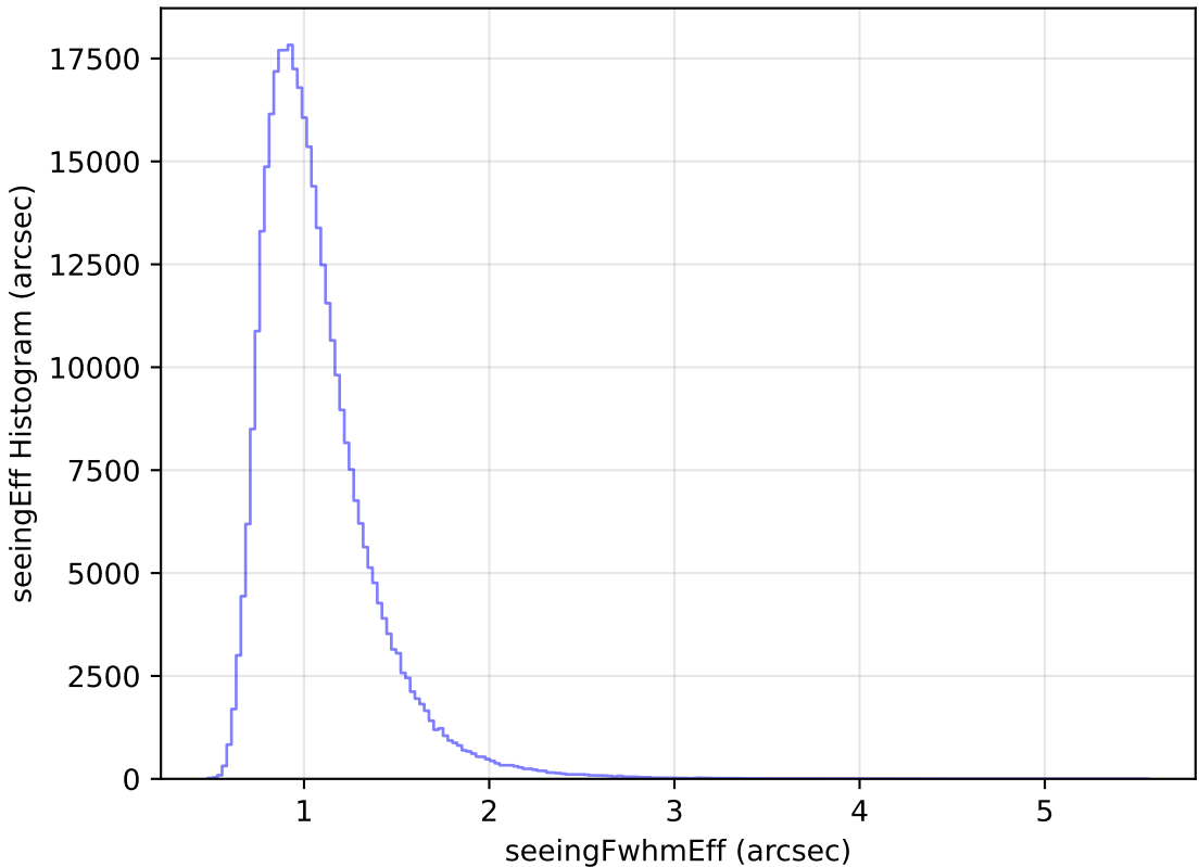
mw_roll_bulge_v3.3_10yrs WFD y band: seeingEff Histogram
