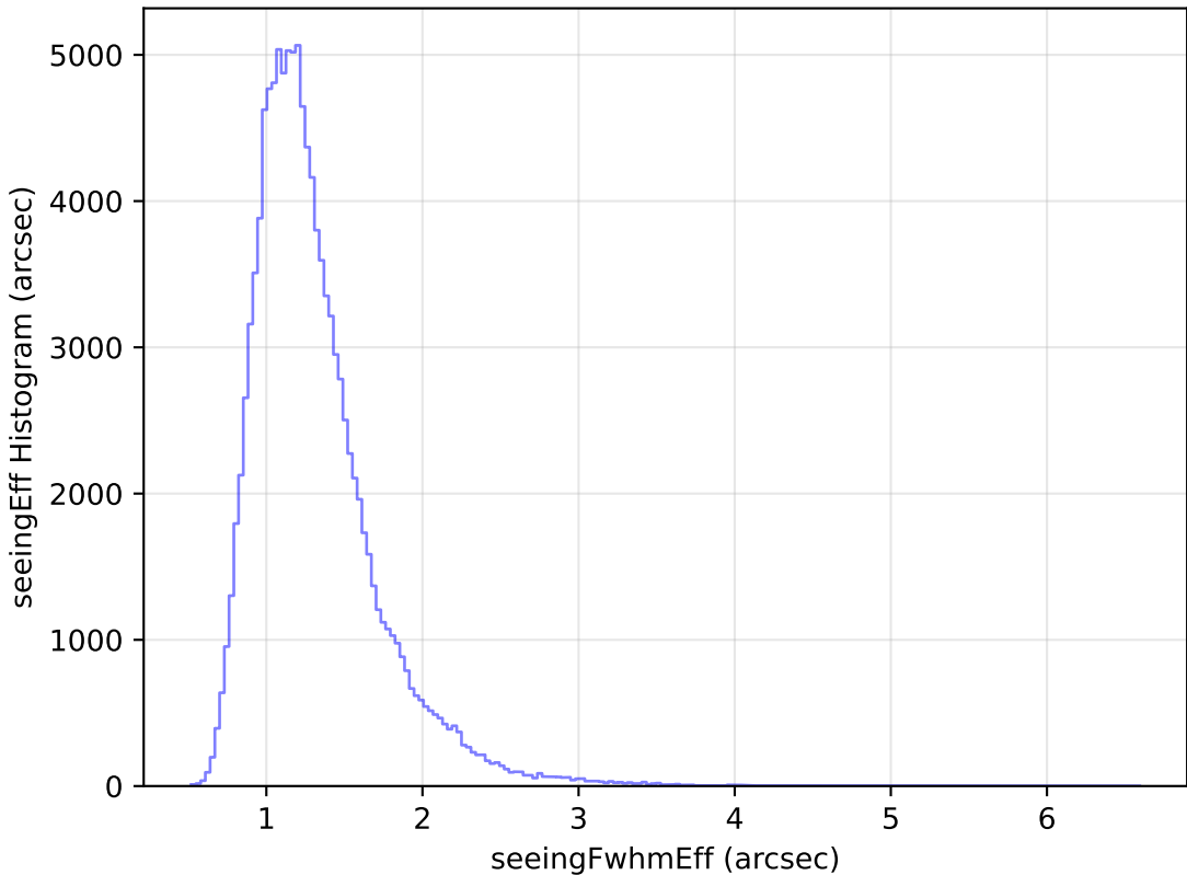
mw_roll_bulge_v3.3_10yrs WFD u band: seeingEff Histogram
