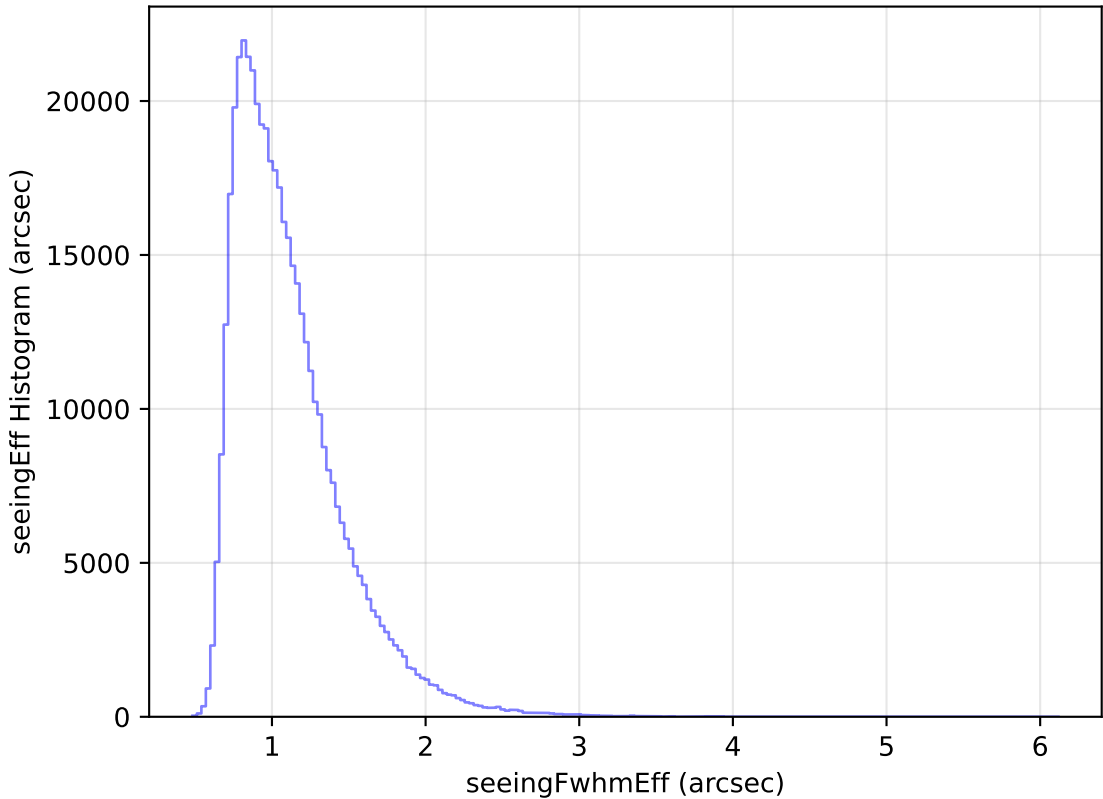
mw_roll_bulge_v3.3_10yrs WFD r band: seeingEff Histogram
