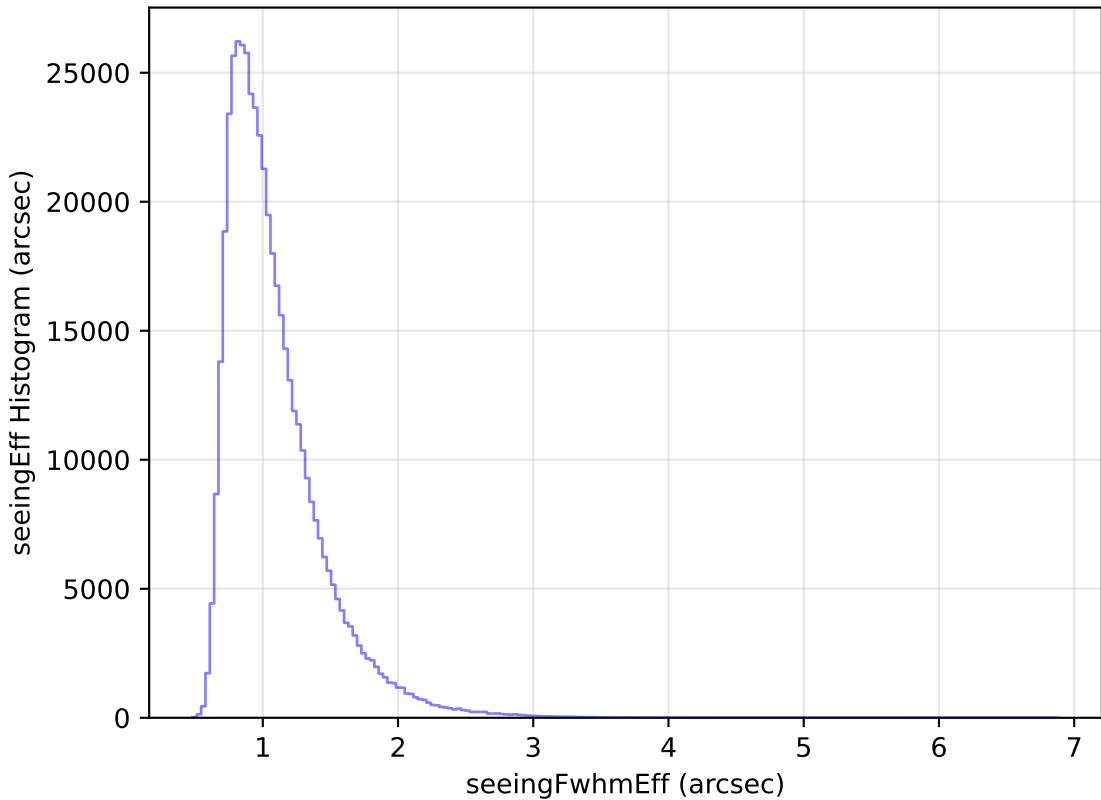
mw_roll_bulge_v3.3_10yrs WFD i band: seeingEff Histogram
