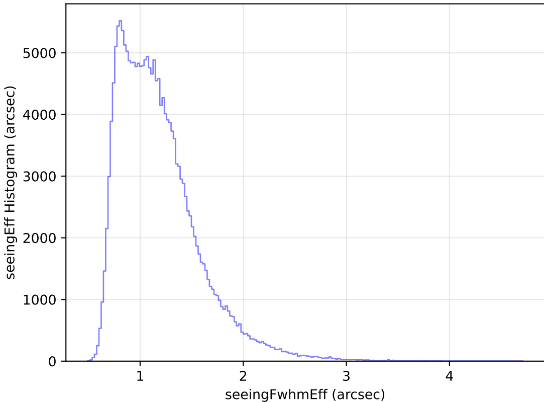
mw_roll_bulge_v3.3_10yrs WFD g band: seeingEff Histogram
