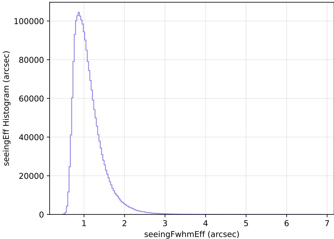
mw_roll_bulge_v3.3_10yrs WFD all bands: seeingEff Histogram
