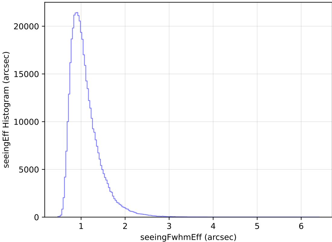
mw_roll_bulge_v3.3_10yrs All sky z band: seeingEff Histogram
