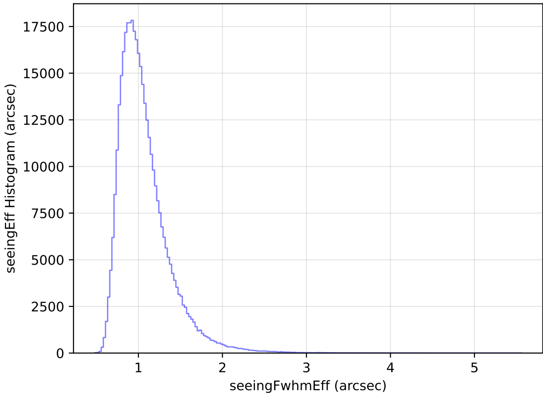
mw_roll_bulge_v3.3_10yrs All sky y band: seeingEff Histogram
