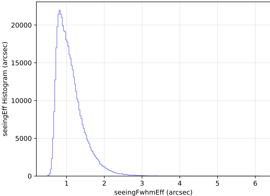
mw_roll_bulge_v3.3_10yrs All sky r band: seeingEff Histogram
